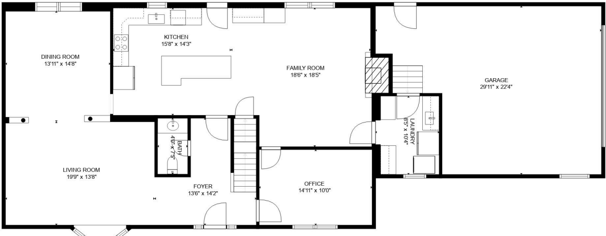
MAIN LEVEL
